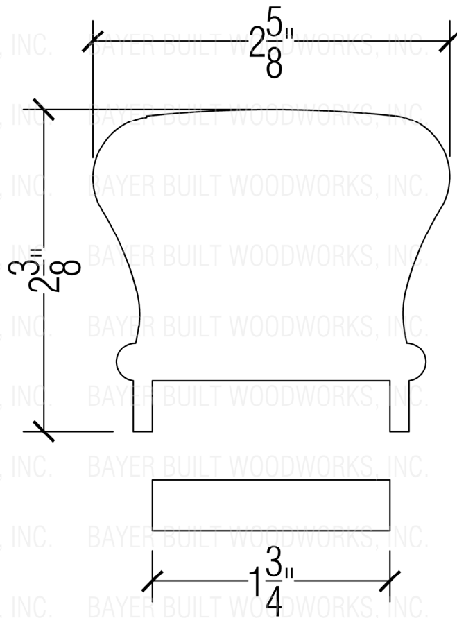
6210P1 RAIL W/ 6007 FILLET
